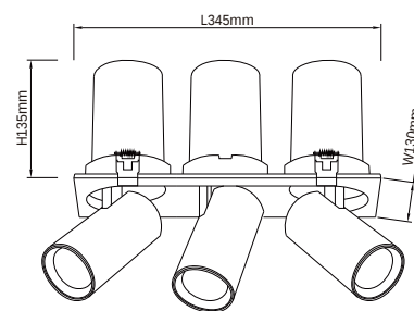
Cut out □ 120*335mm
