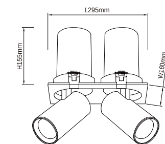
Cut out □140*280mm
