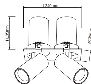
Cut out □ 120*230mm
